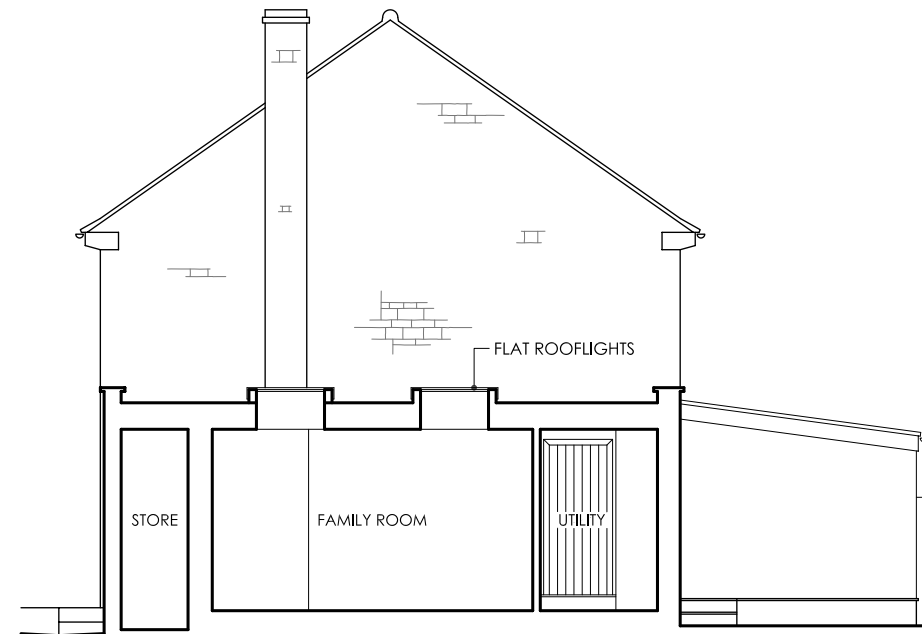
SOUTH WEST SECTION ELEVATION
