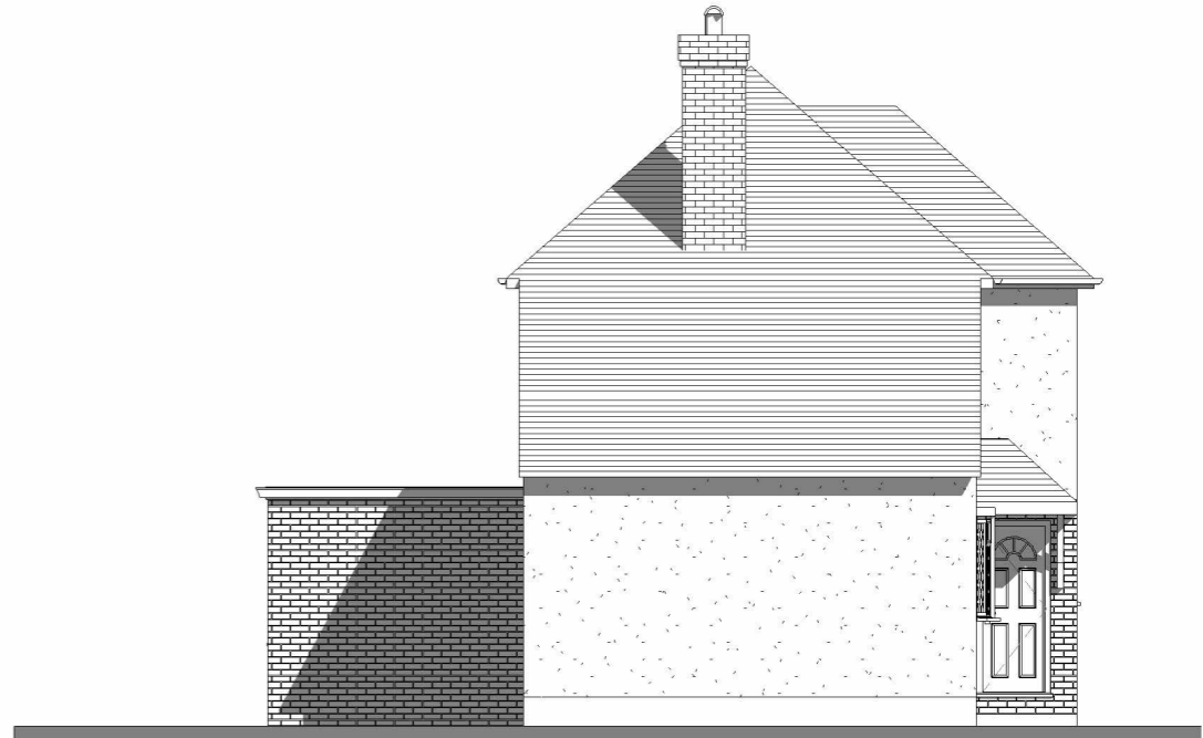
2 Existing Side 1 Elevation 1 : 100
