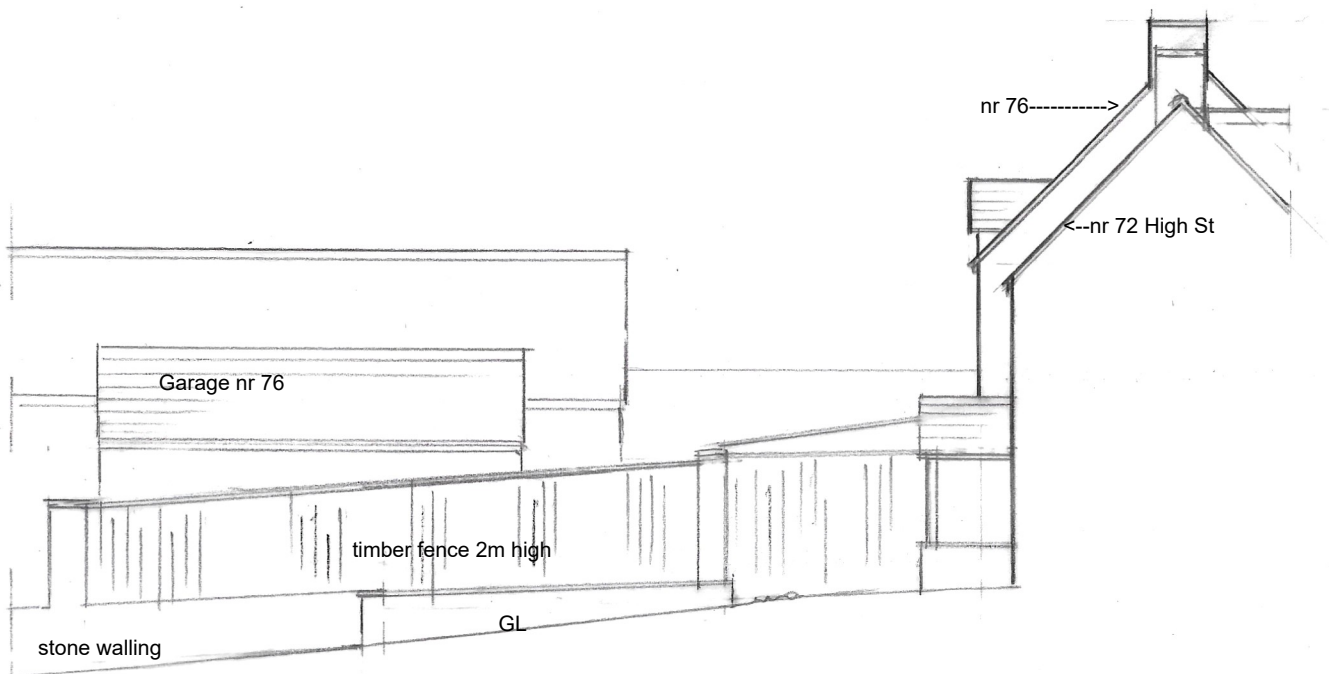
EAST ELEVATION
