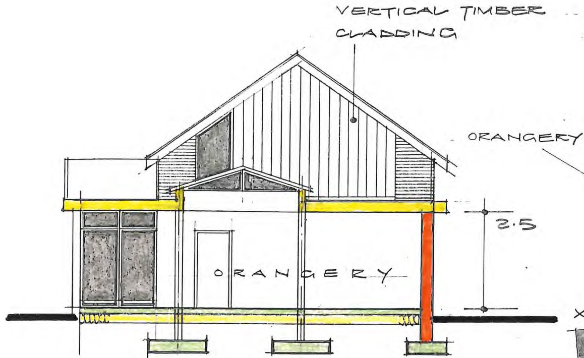
SECTION THRO' ORANGERY X.X SCALE 1 TO 100
