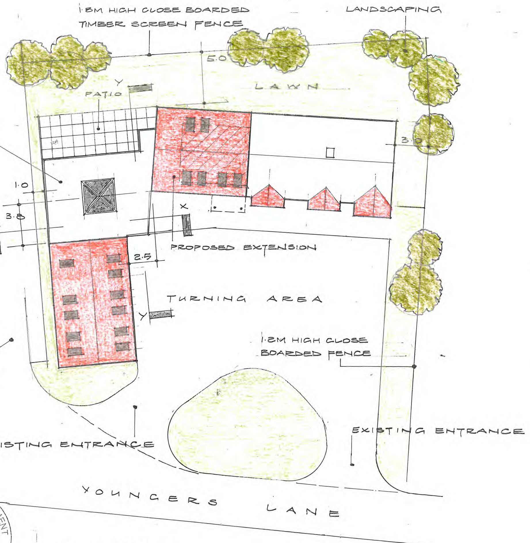
SITE LAYOUT SCALE 1 TO 200
