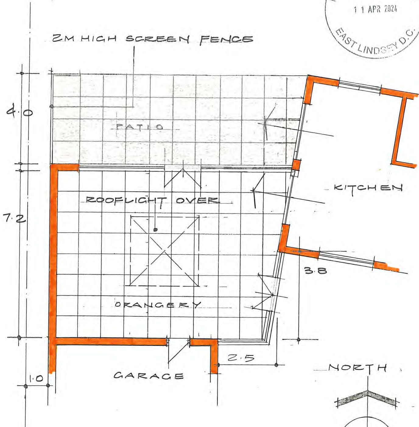
PLAN OF ORANGERY
