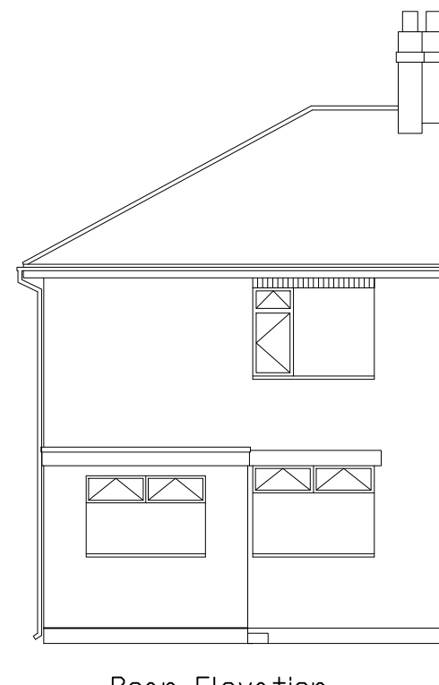
Rear Elevation
