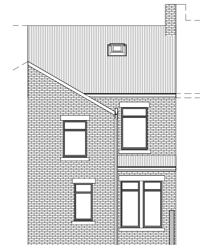
8 Rear Elevation 1 : 100
