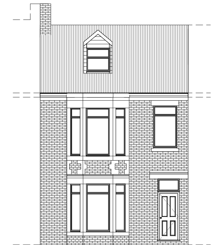
5 Front Elevation 1 : 100
