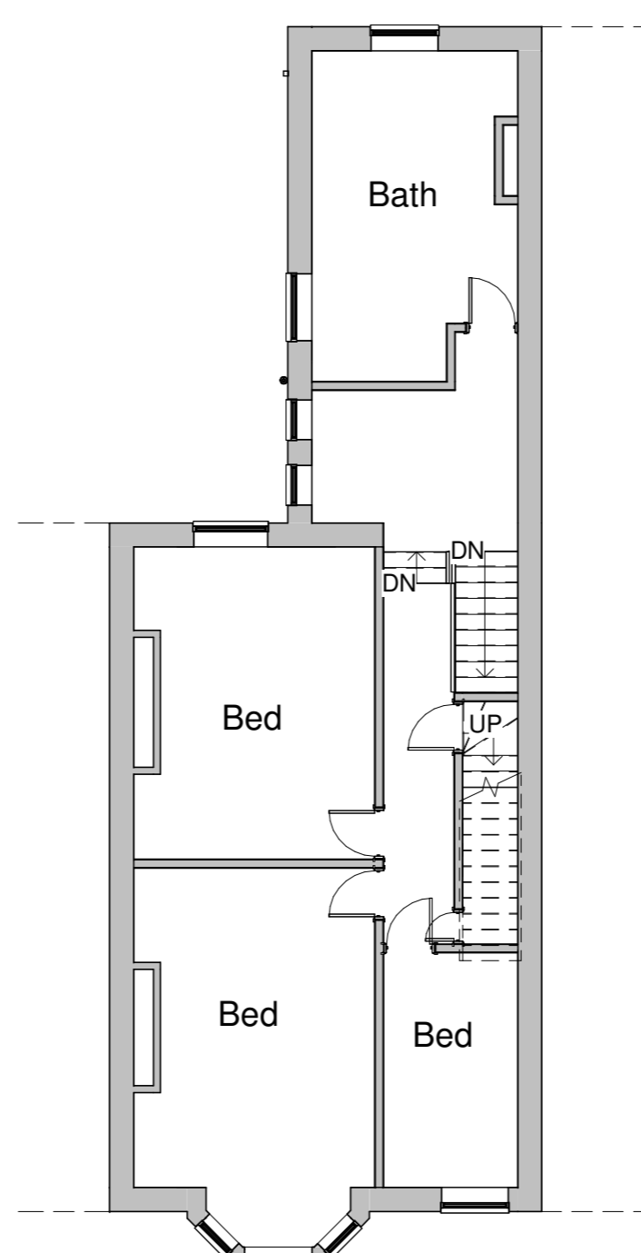
3 First Floor 1 : 100
