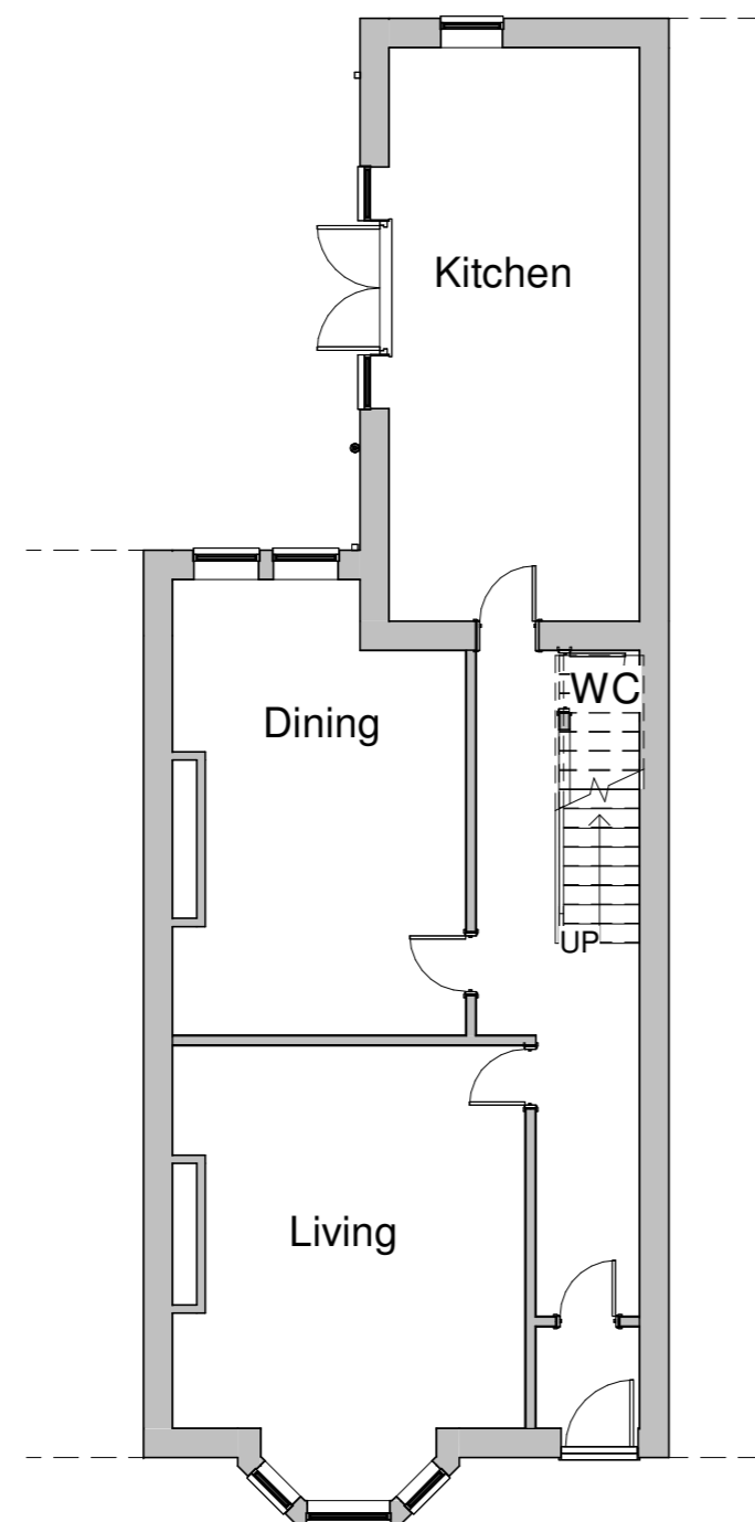
2 Ground Floor 1 : 100
