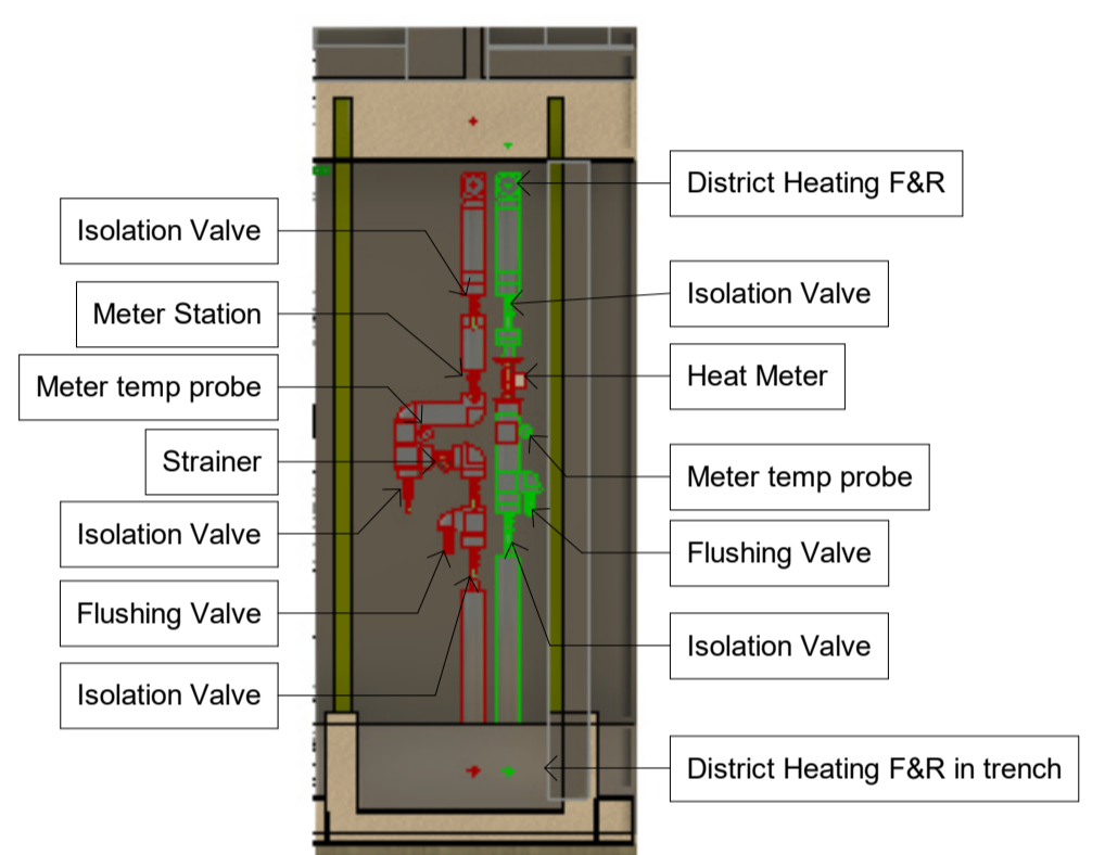
2 District Heating Section 1 1 : 50
