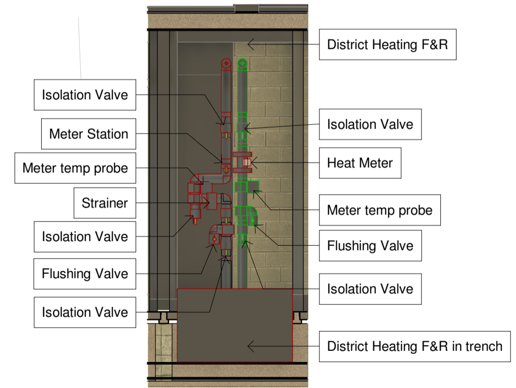
2 District Heating Section 1 1 : 50
