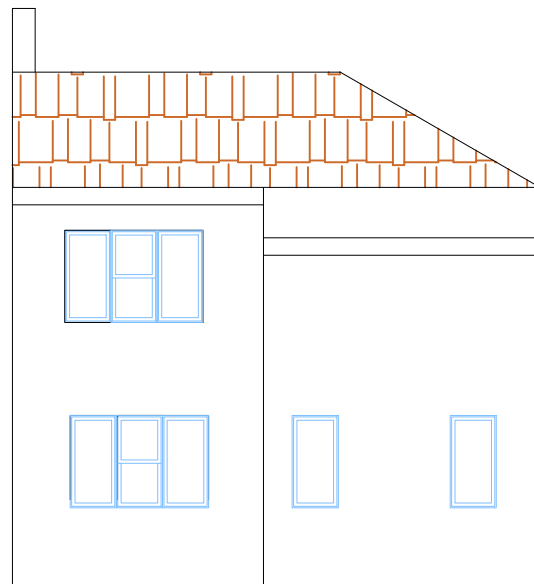
Existing Left Side Elevation
