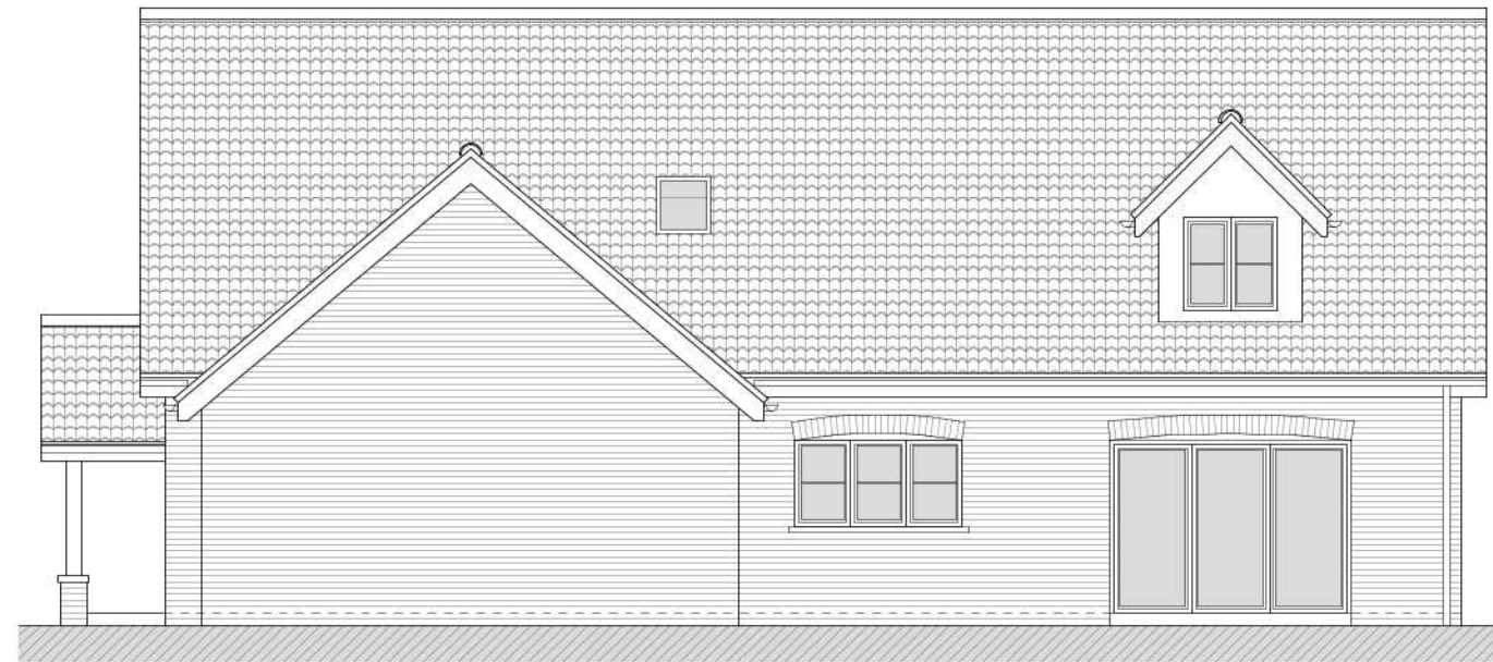
SIDE / SOUTHERN ELEVATION
