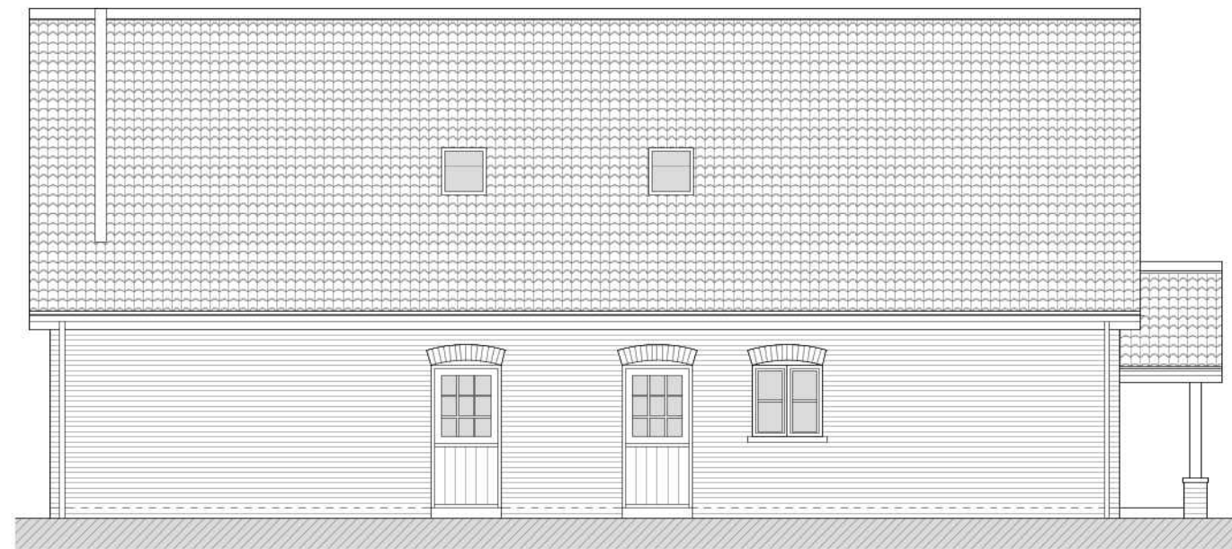
SIDE / NORTHERN ELEVATION
