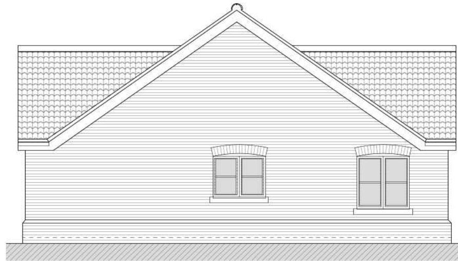
SIDE / SOUTHERN ELEVATION
