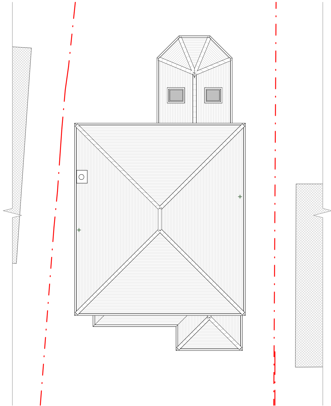
Roof Plan
