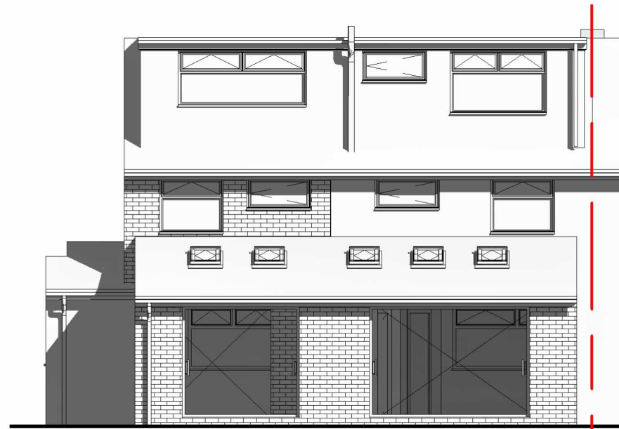
4 Proposed N-West Elevation 1 : 100
