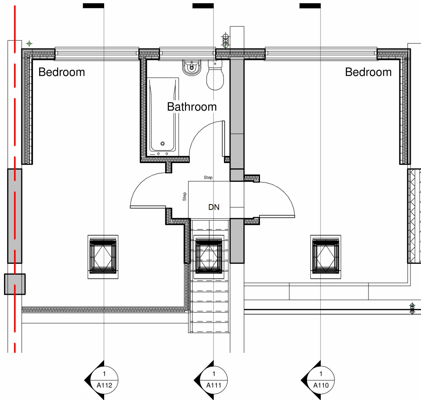
1 Proposed Second Floor 1 : 50
