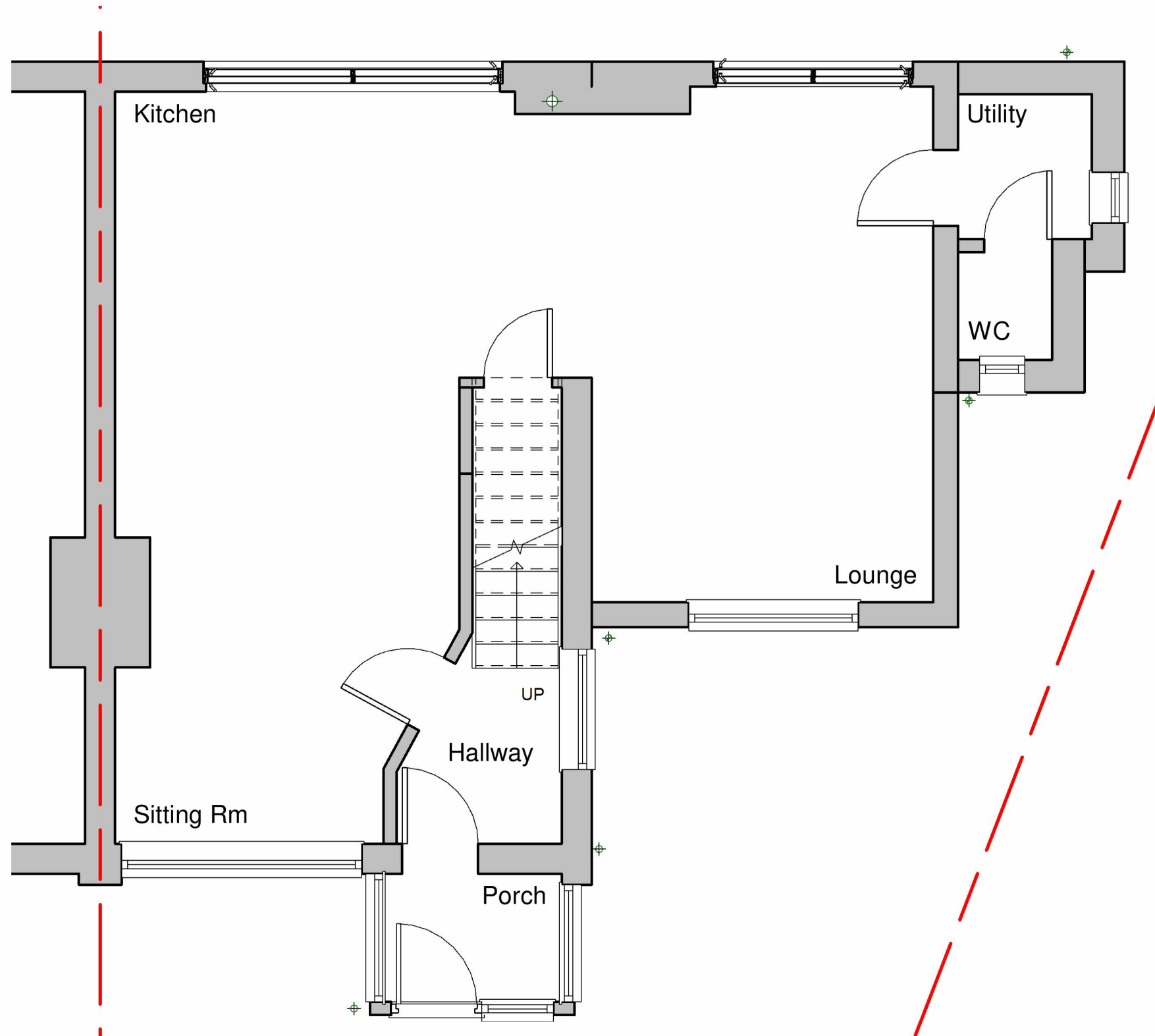
1 Existing Ground Floor 1 : 50
