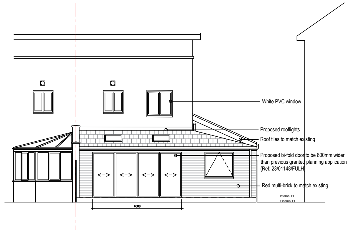
01 PROPOSED SOUTH EAST ELEVATION 104 1:100
