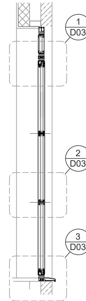
Vertical section through door
