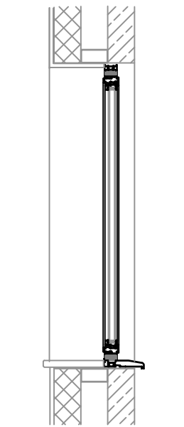
Vertical section through window
