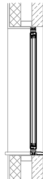
Vertical section through window
