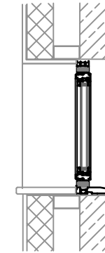
Vertical section through window
