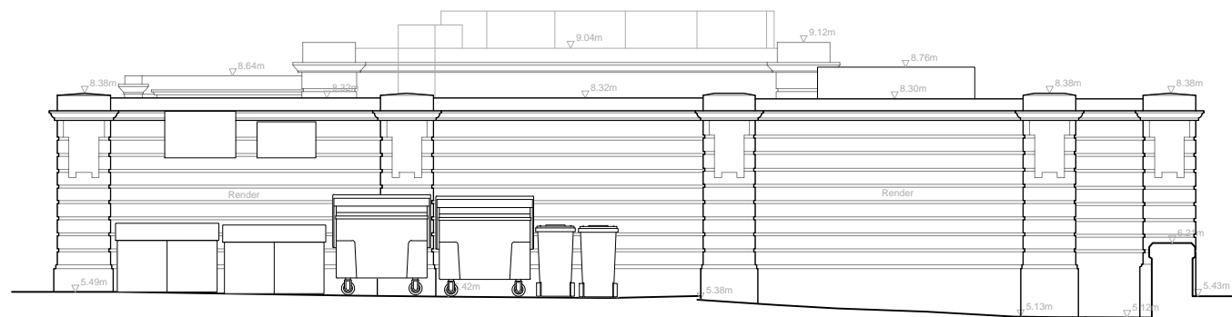
EXISTING SOUTH (ROAD) ELEVATION
