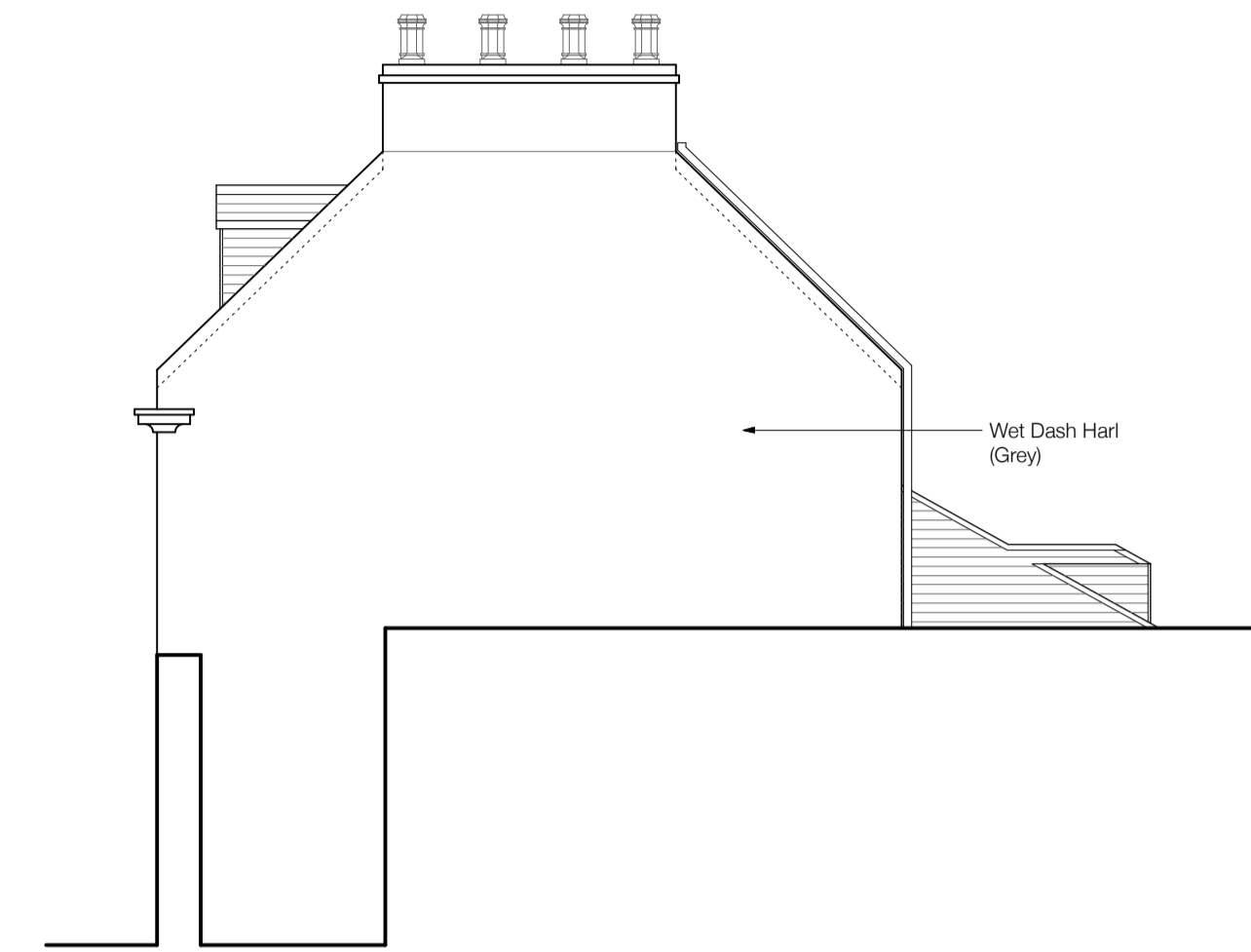
East Elevation 1:100
