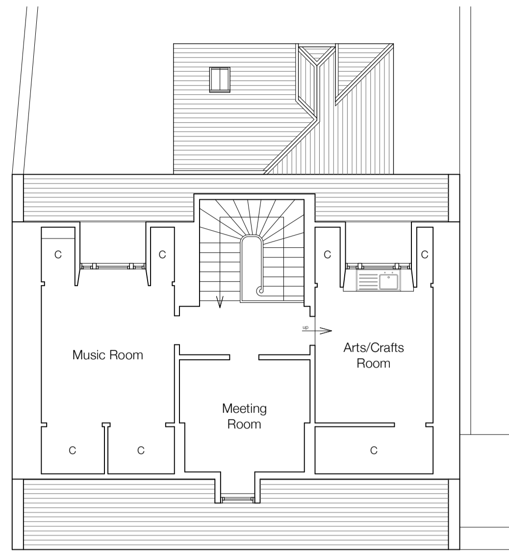
Second Floor Plan 1:100
