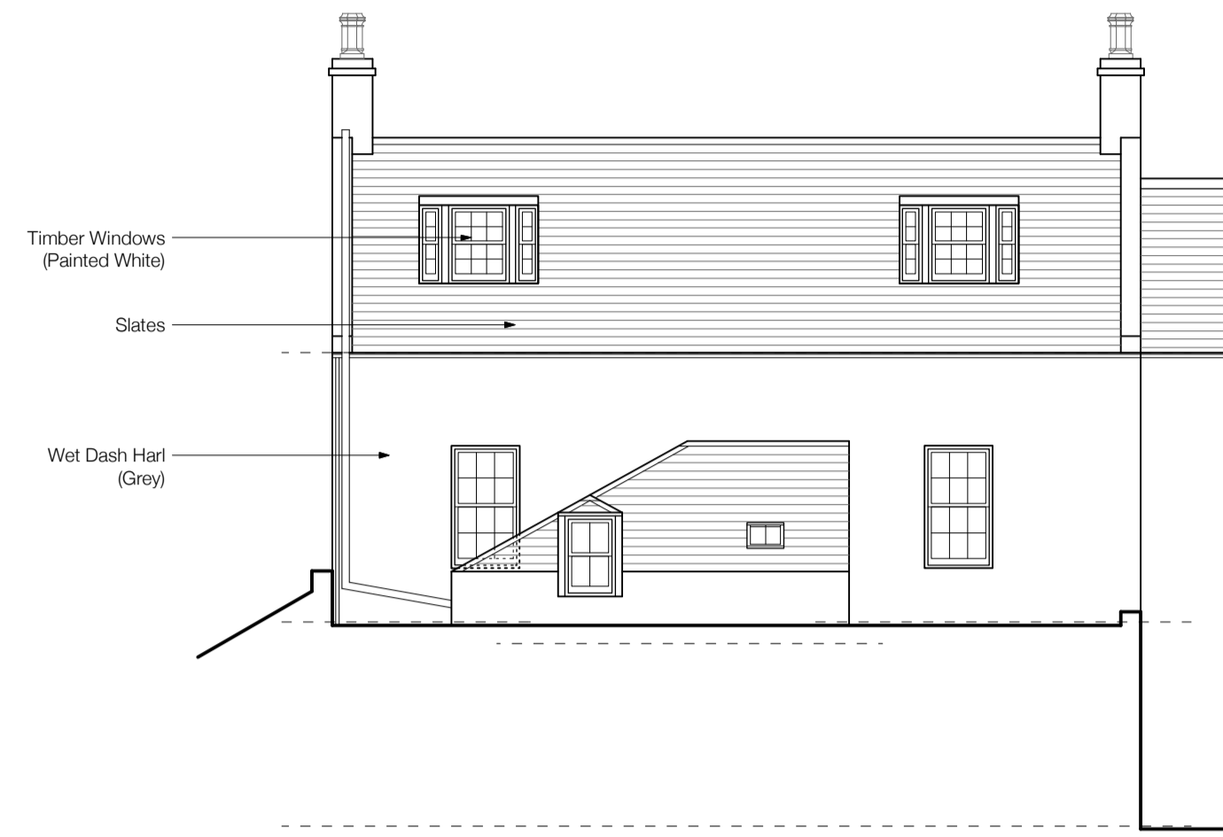
North Elevation 1:100
