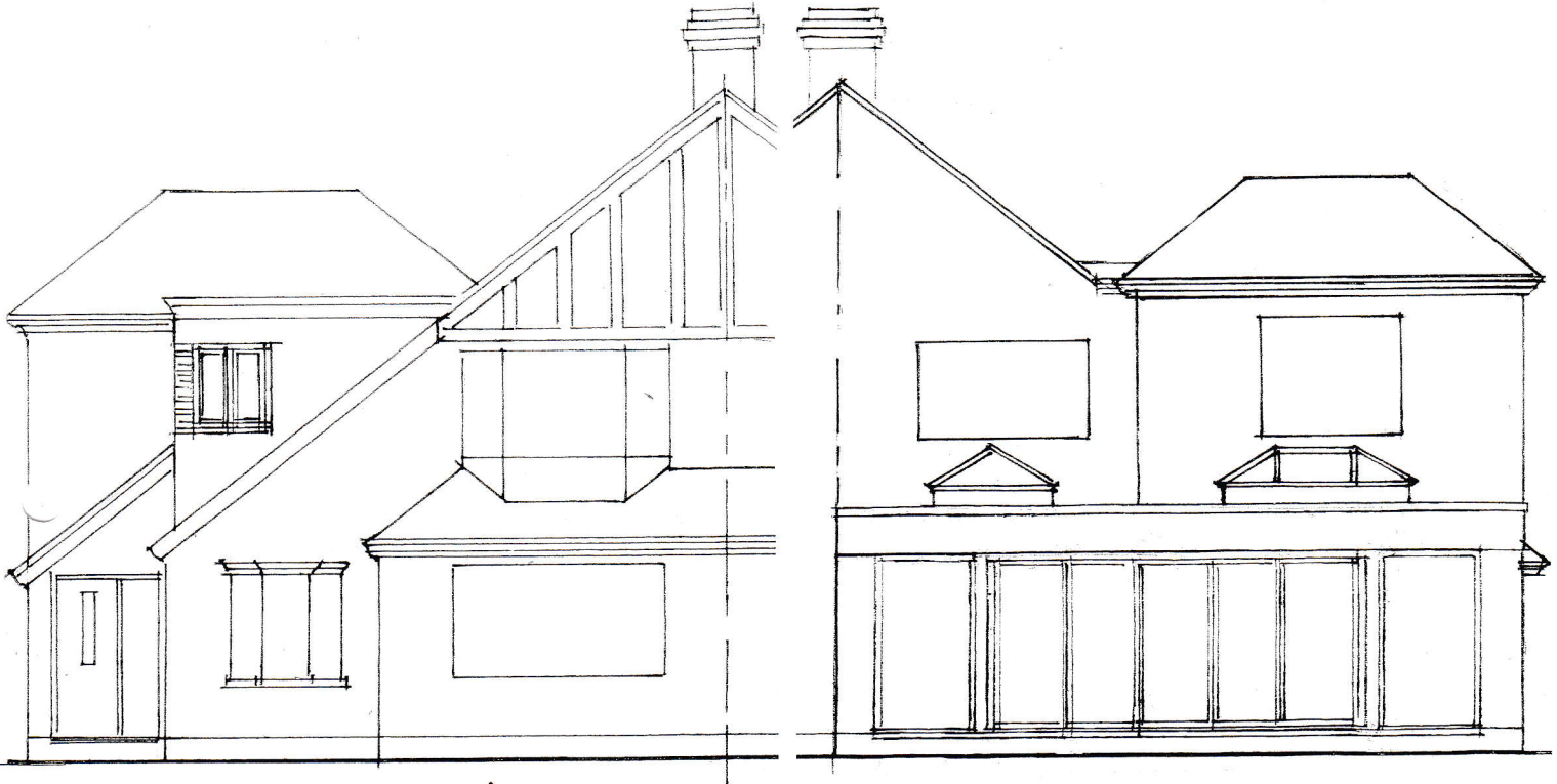
FRONT ELEVATION
