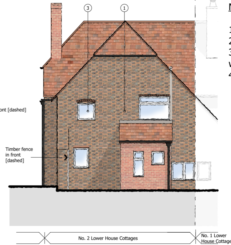
SOUTH-WEST ELEVATION 1:100
