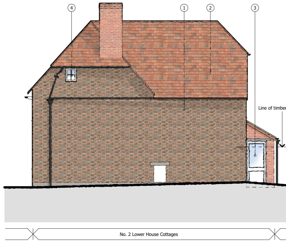
NORTH-WEST ELEVATION 1:100
