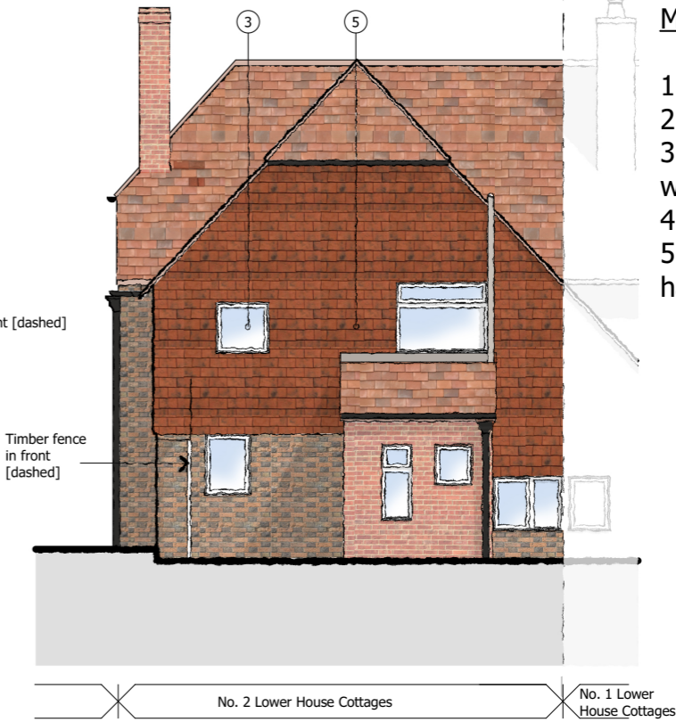
SOUTH-WEST ELEVATION 1:100
