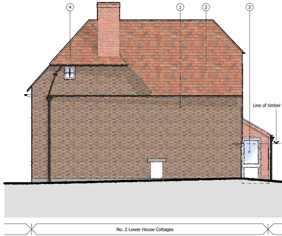
NORTH-WEST ELEVATION 1:100
