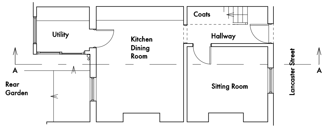
Ground Floor Plan @ 1:100 (A3)
