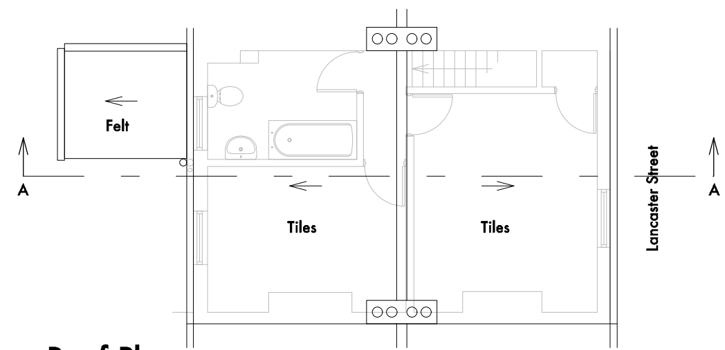
Roof Plan @ 1:100 (A3)
