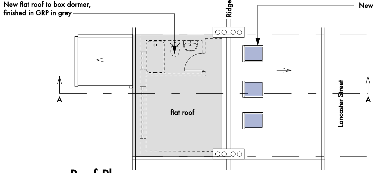
Roof Plan @ 1:100 (A3)
