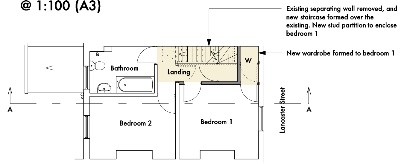
First Floor Plan @ 1:100 (A3)
