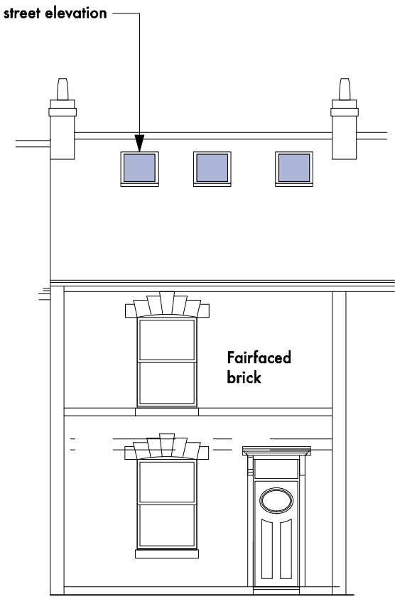
East (Street) Elevation @ 1:100 (A3)
