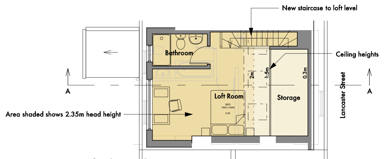
Loft Floor Plan @ 1:100 (A3)
