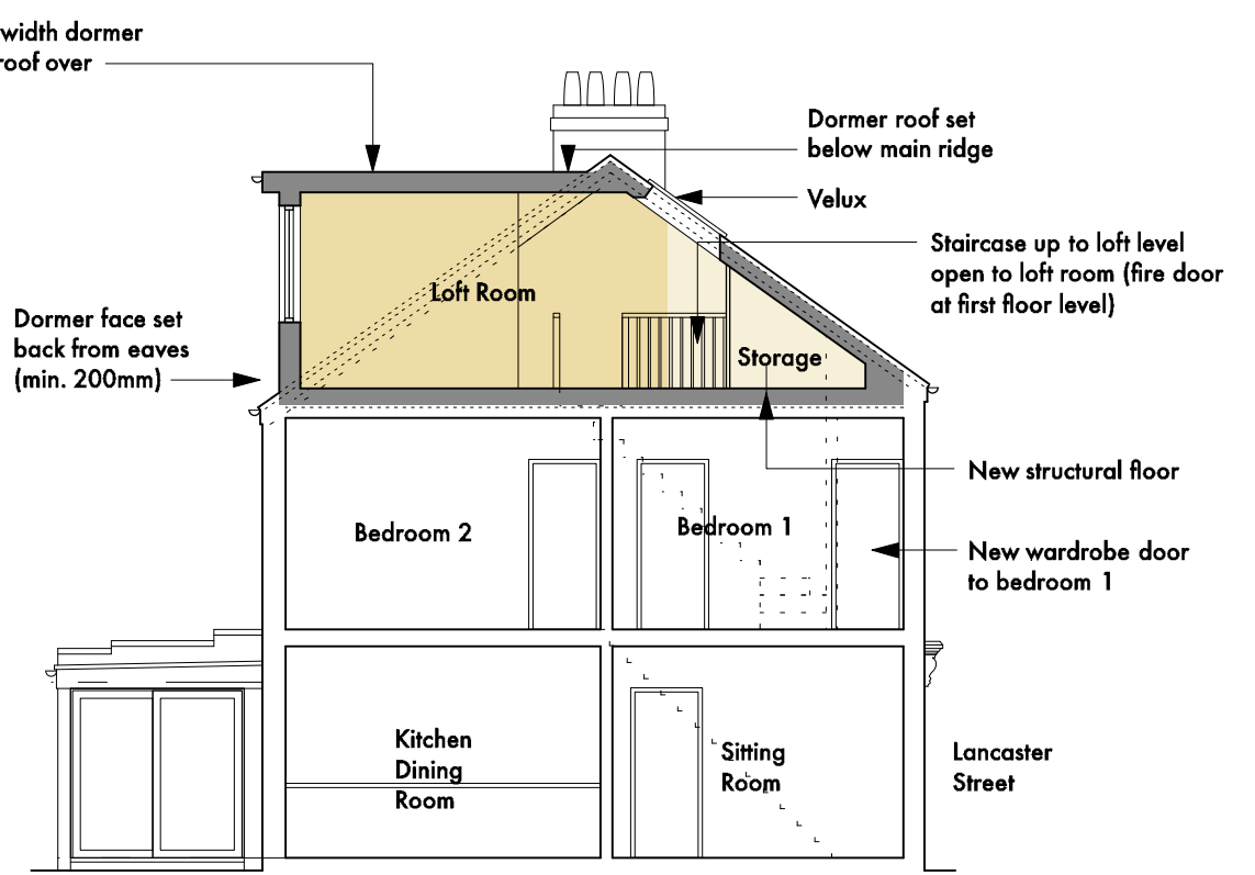
Section A-A @ 1:100 (A3)
