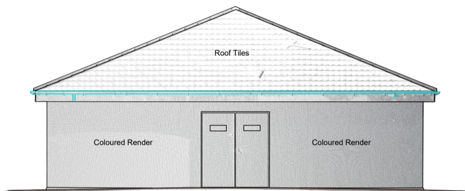
West Elevation
