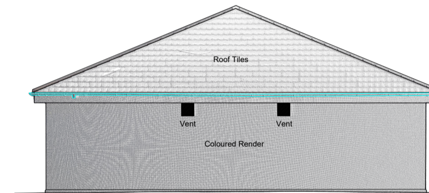
East Elevation
