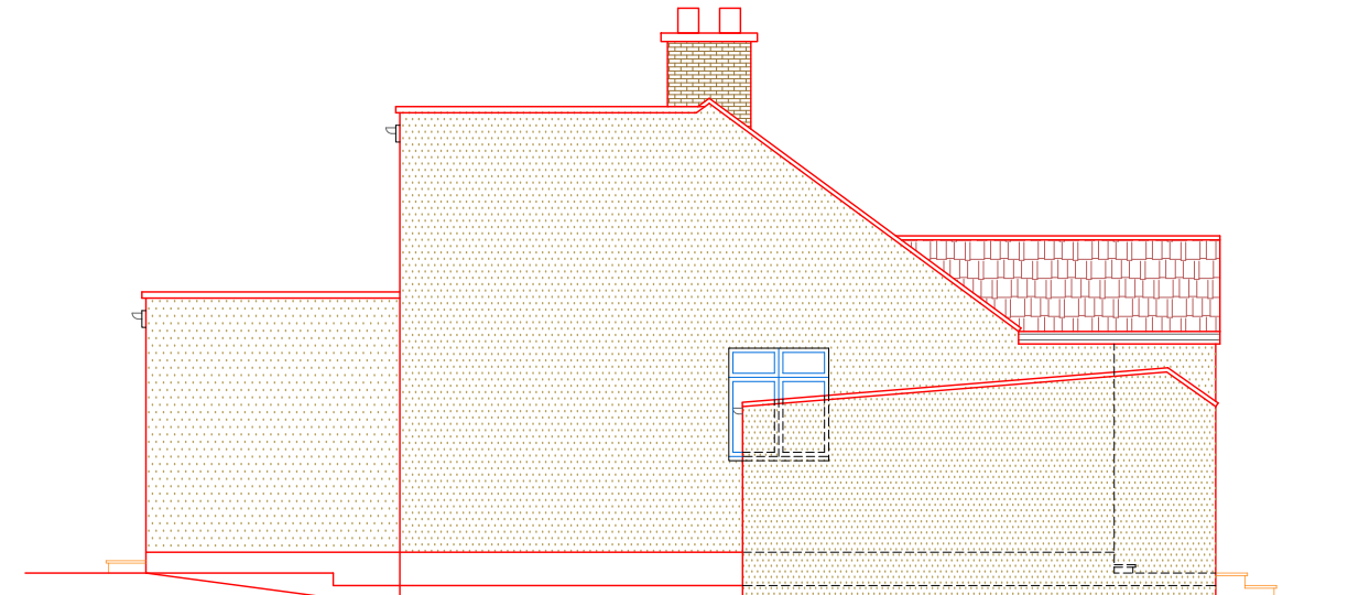
EXISTING SIDE ELEVATION-2
