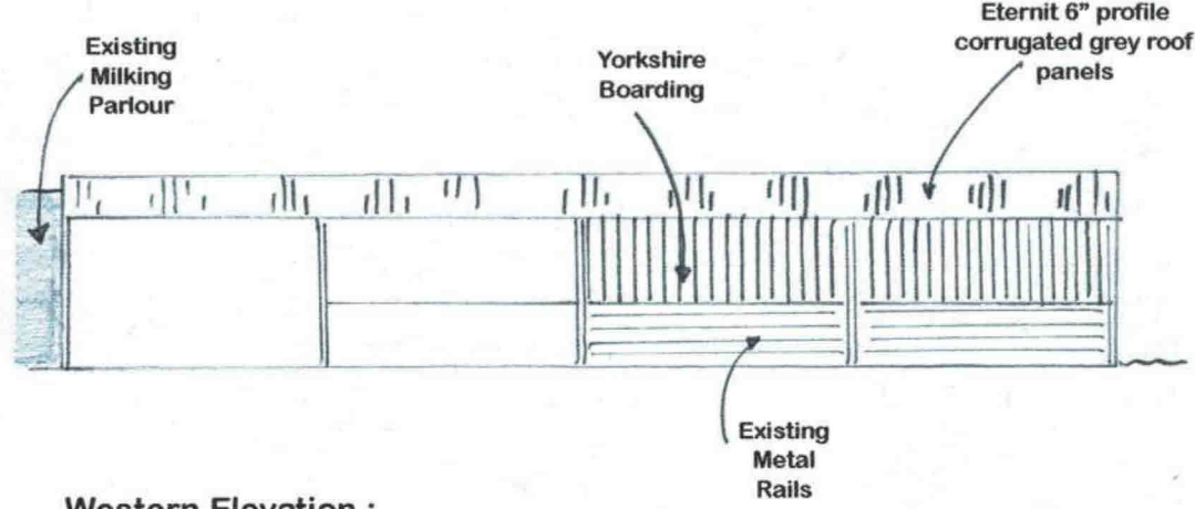
Western Elevation :
