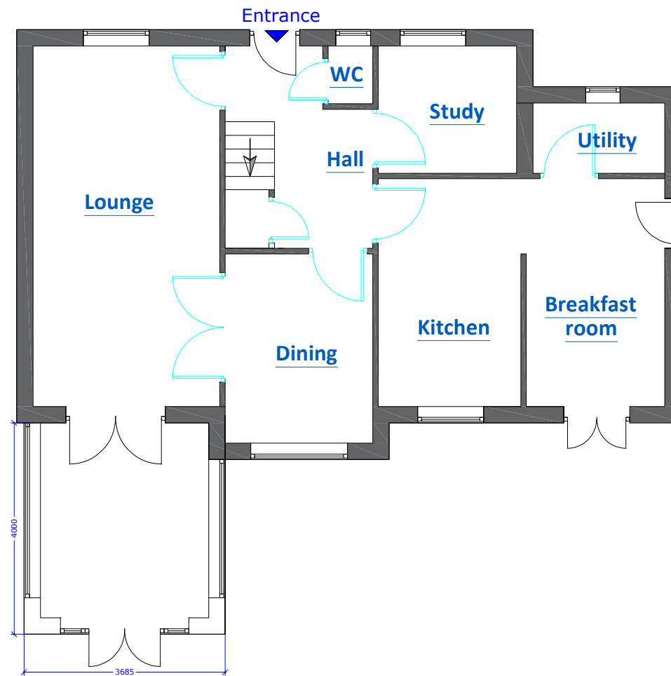
Proposed Floorplan
