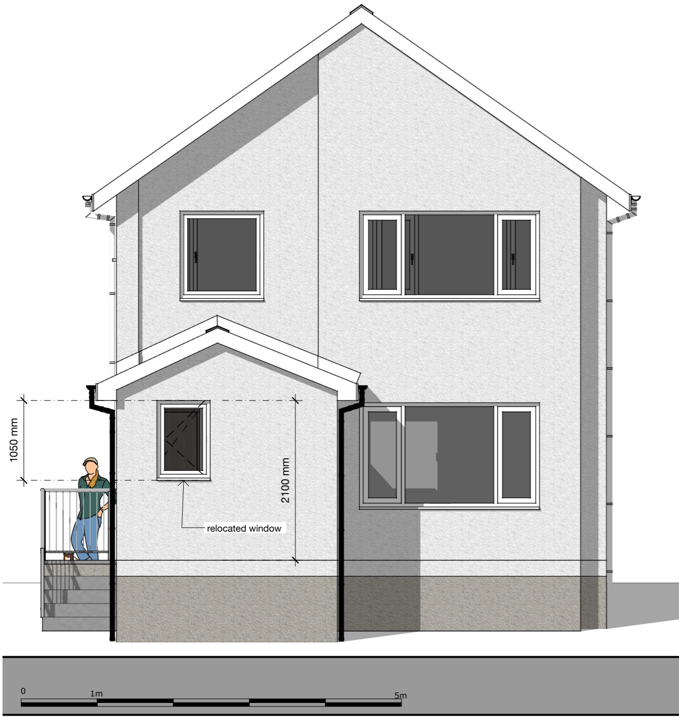
P 3 :: PROPOSED FRONT ELEVATION scale: 1:50
