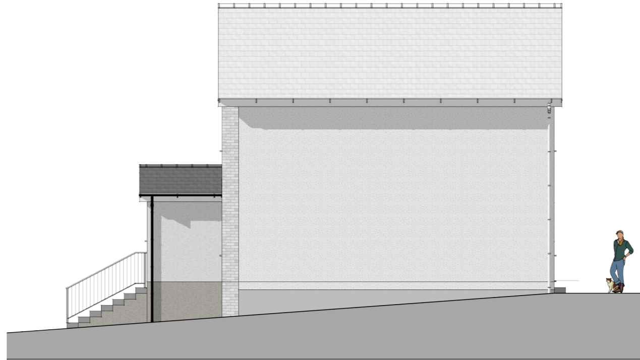
P :: PREVIOUSLY APPROVED SIDE ELEVATION 1 scale: 1:100
