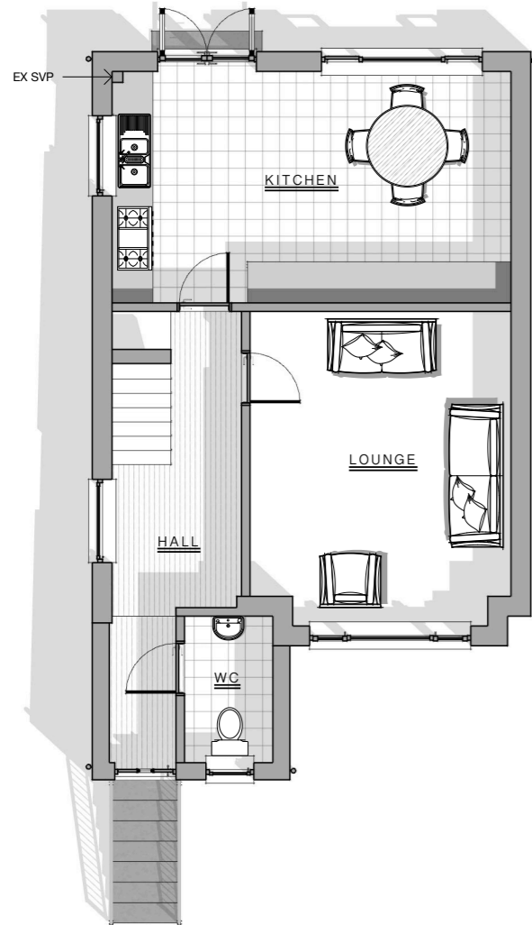
P :: PREVIOUSLY APPROVED GROUND FLOOR PLAN 1 scale: 1:100
