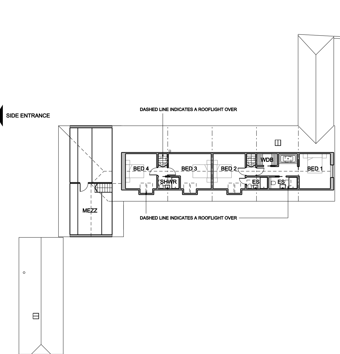
FIRST FLOOR GIA 78.5 SQM (EXCL. GARAGE MEZZ)
