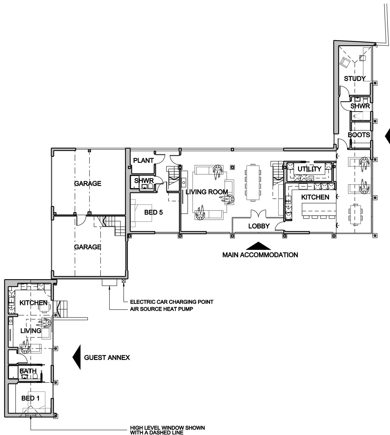
GROUND FLOOR GIA 224.0 SQM (EXCL. GARAGE) TOTAL GIA 302.5 SQM
