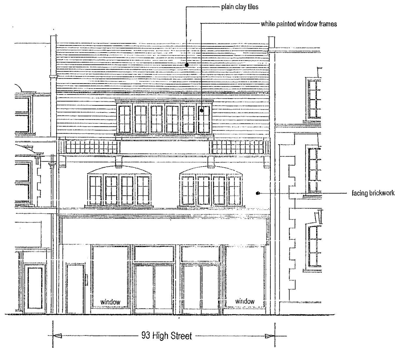
Front elevation
