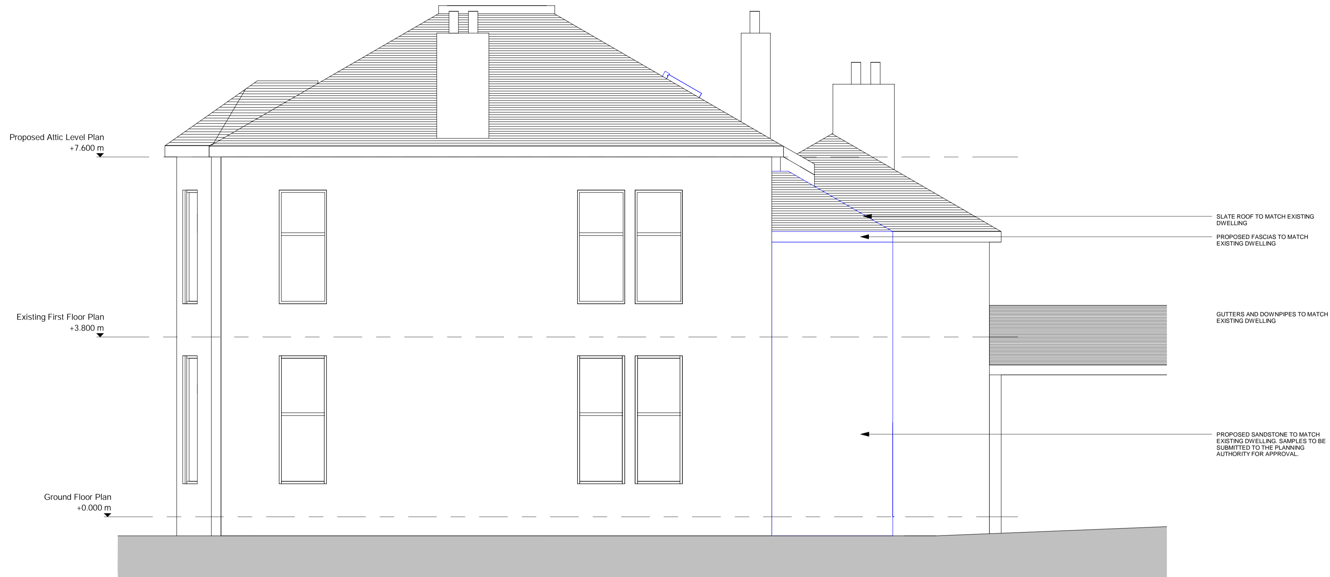
Proposed Side Elevation 1 (NITHSDALE ROAD)
