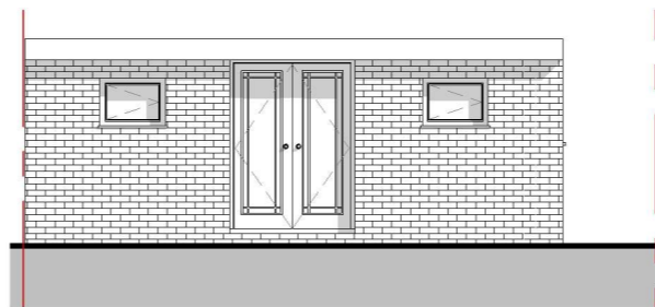
Front (East) 1 : 100
