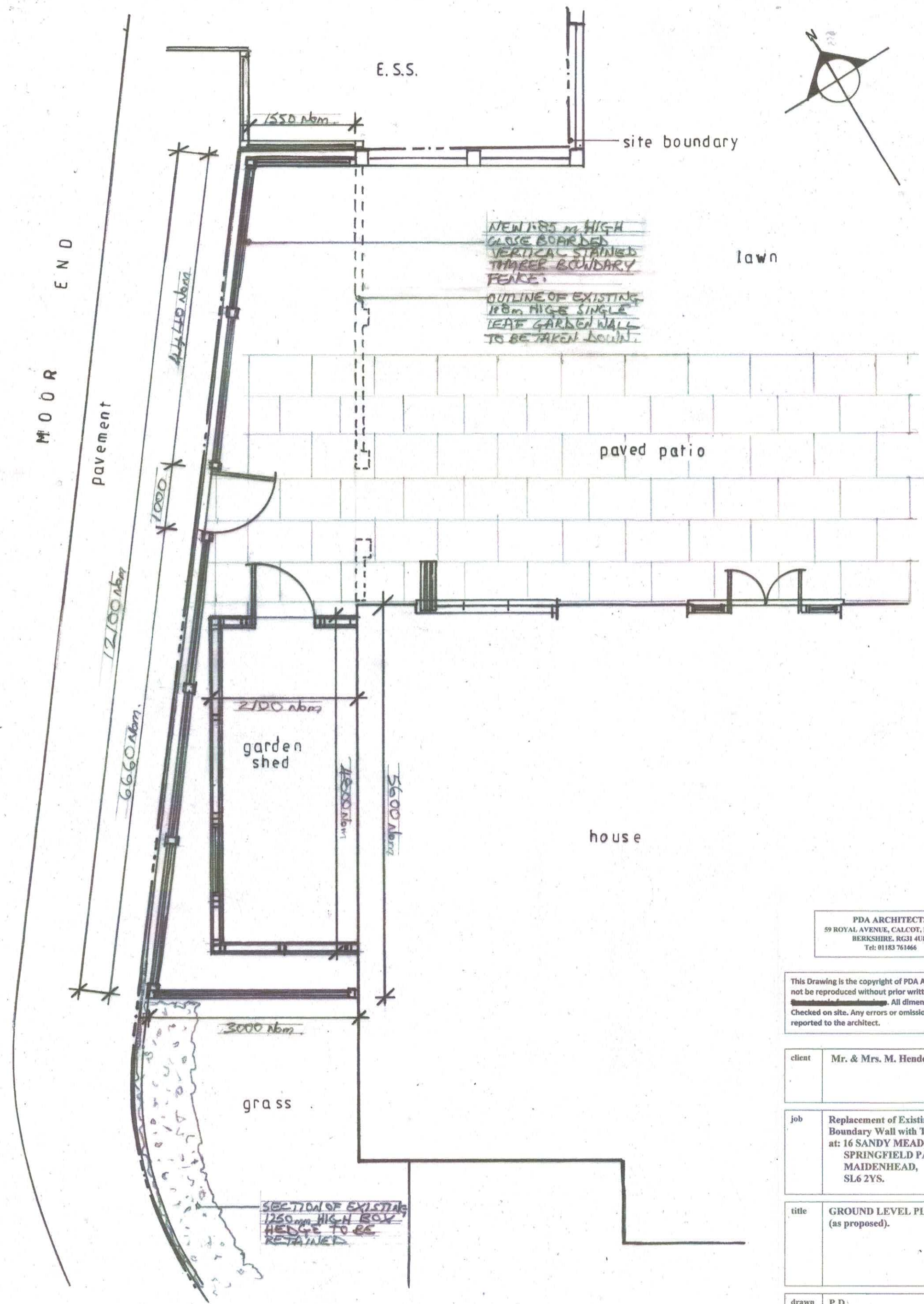
1 GROUND LEVEL PLAN as proposed 1:50
