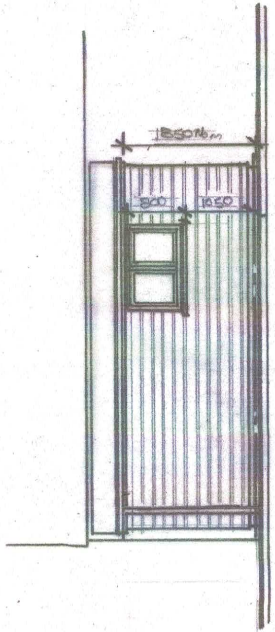
2 SIDE (north west) ELEVATION 1:50
