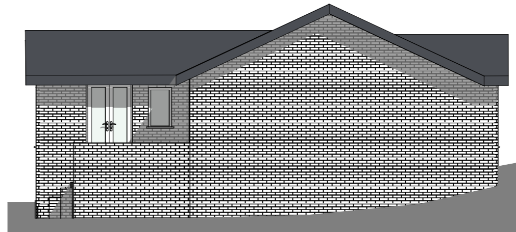
EXISTING SIDE (SOUTH ELEVATION) 1:100
