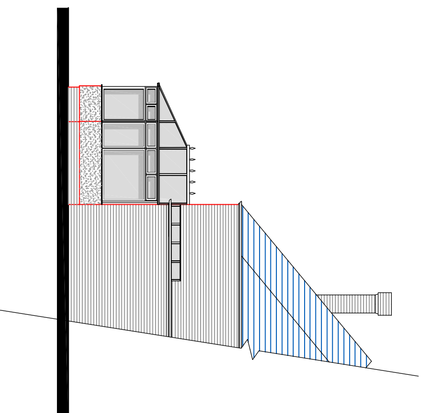
EAST ELEVATION
