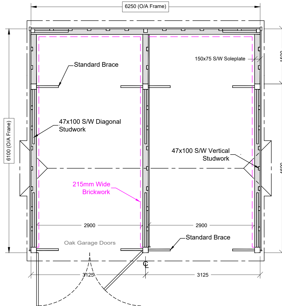
Floor Plan
