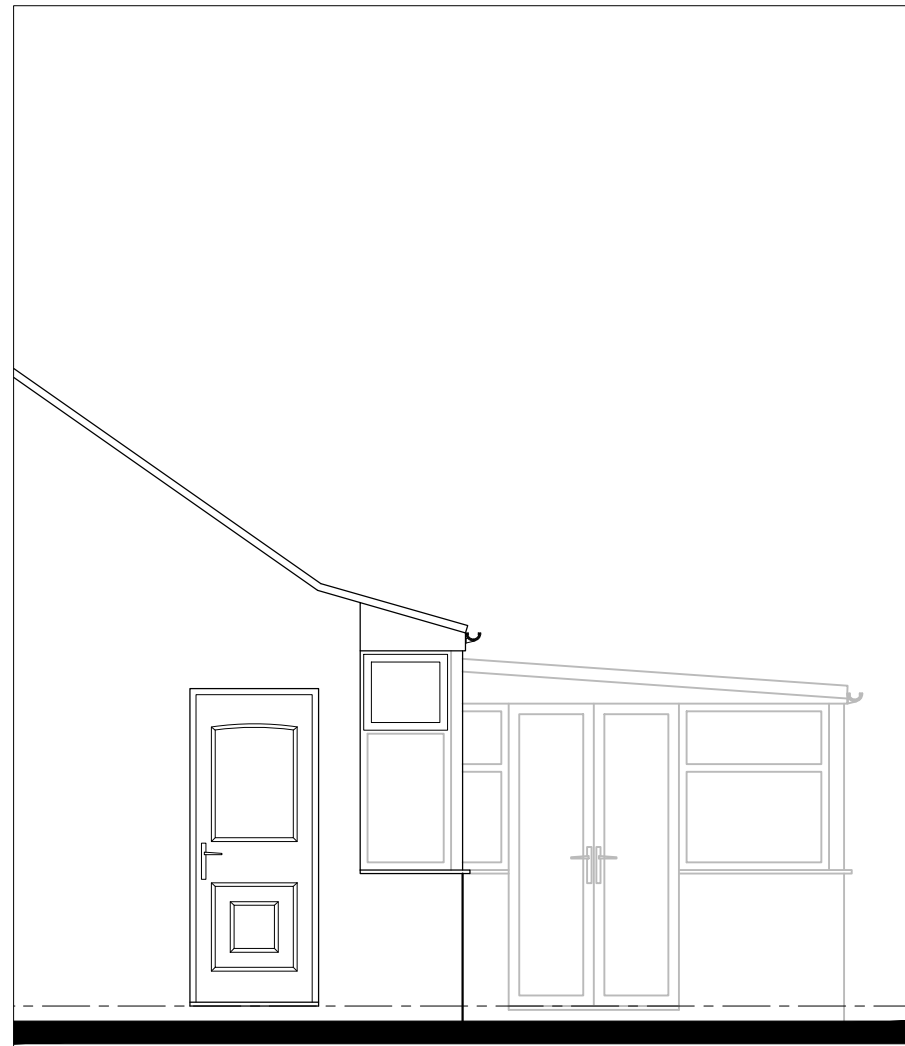
SIDE ELEVATION AS EXISTING
