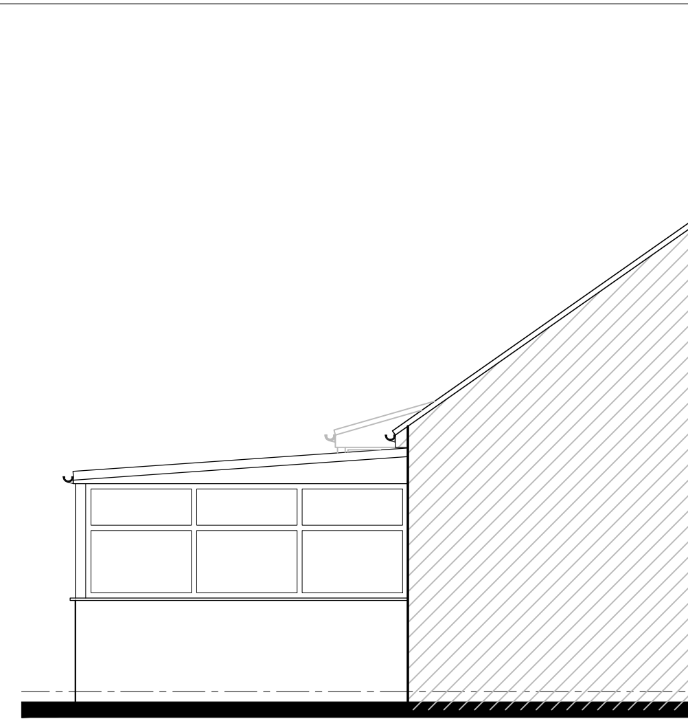
BOUNDARY SIDE ELEVATION AS EXISTING
