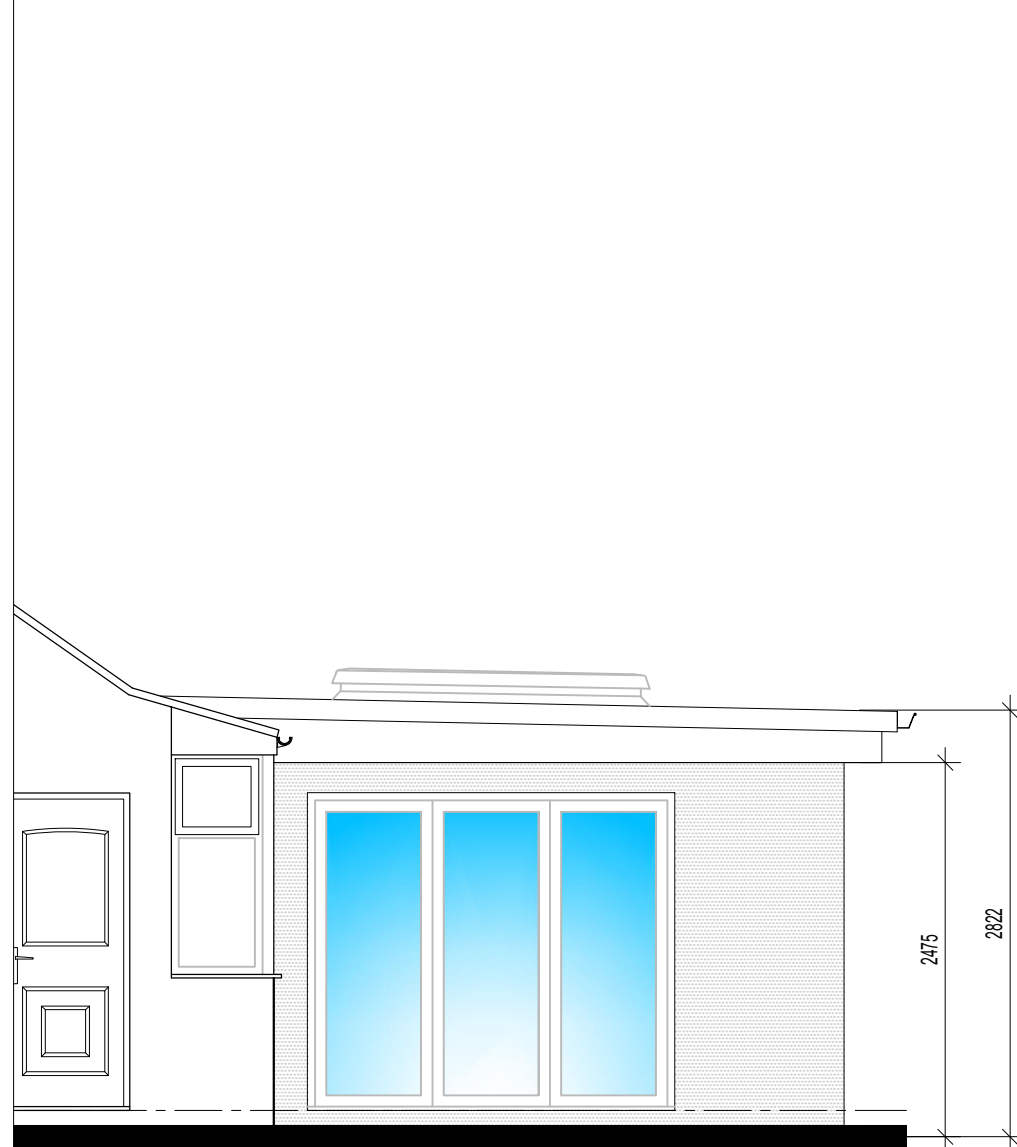
SIDE ELEVATION AS PROPOSED
