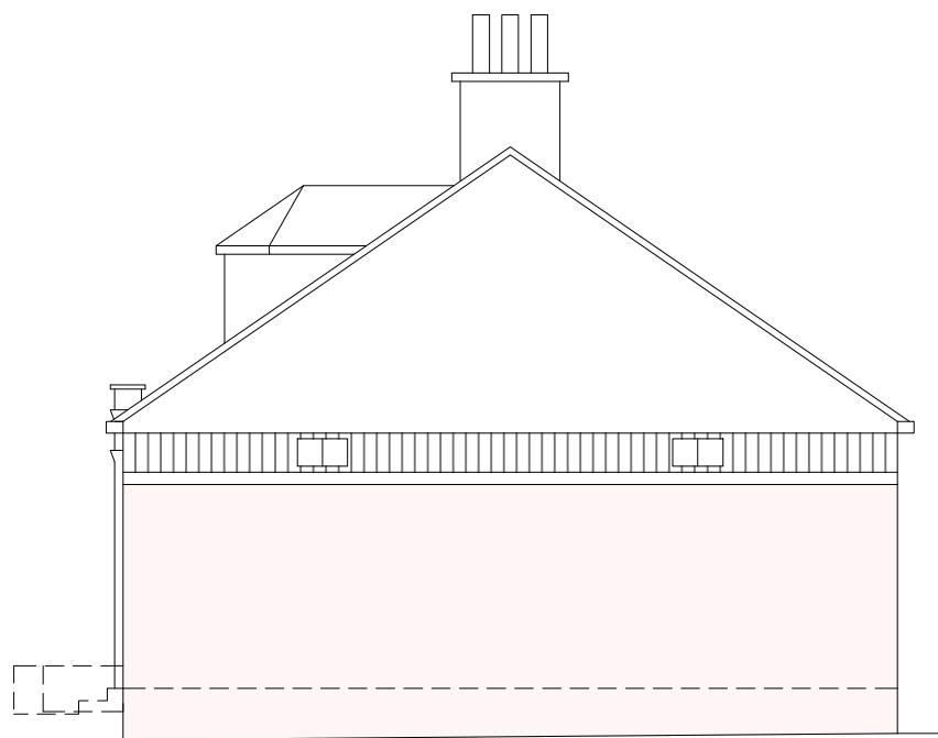
South Elevation
