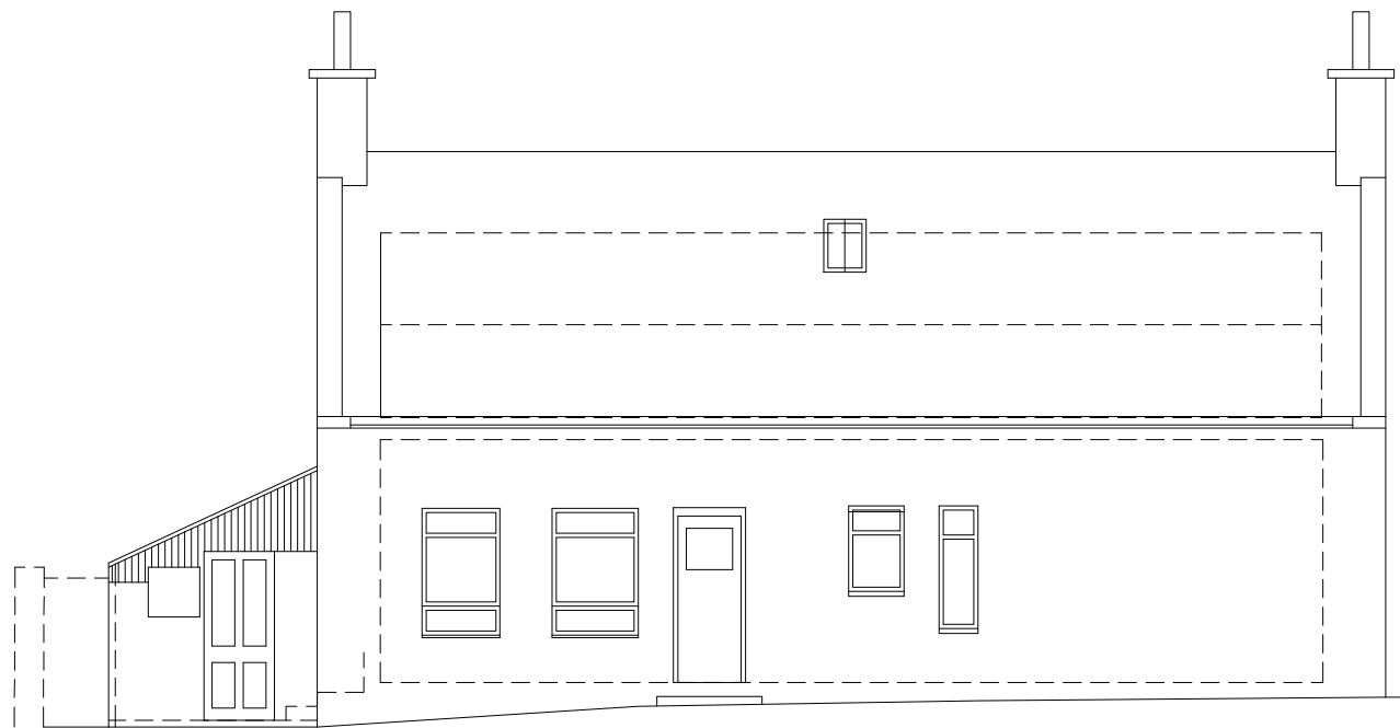
East Elevation
