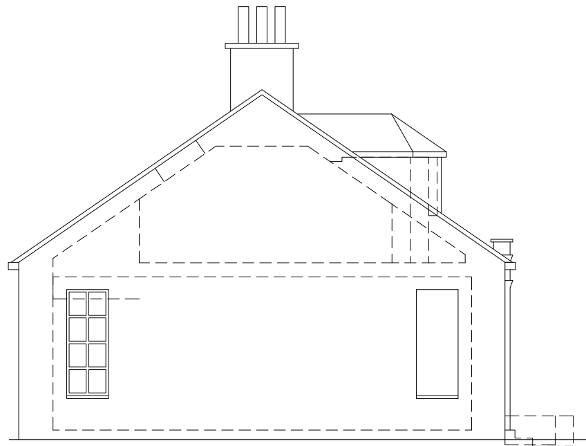
North Elevation
