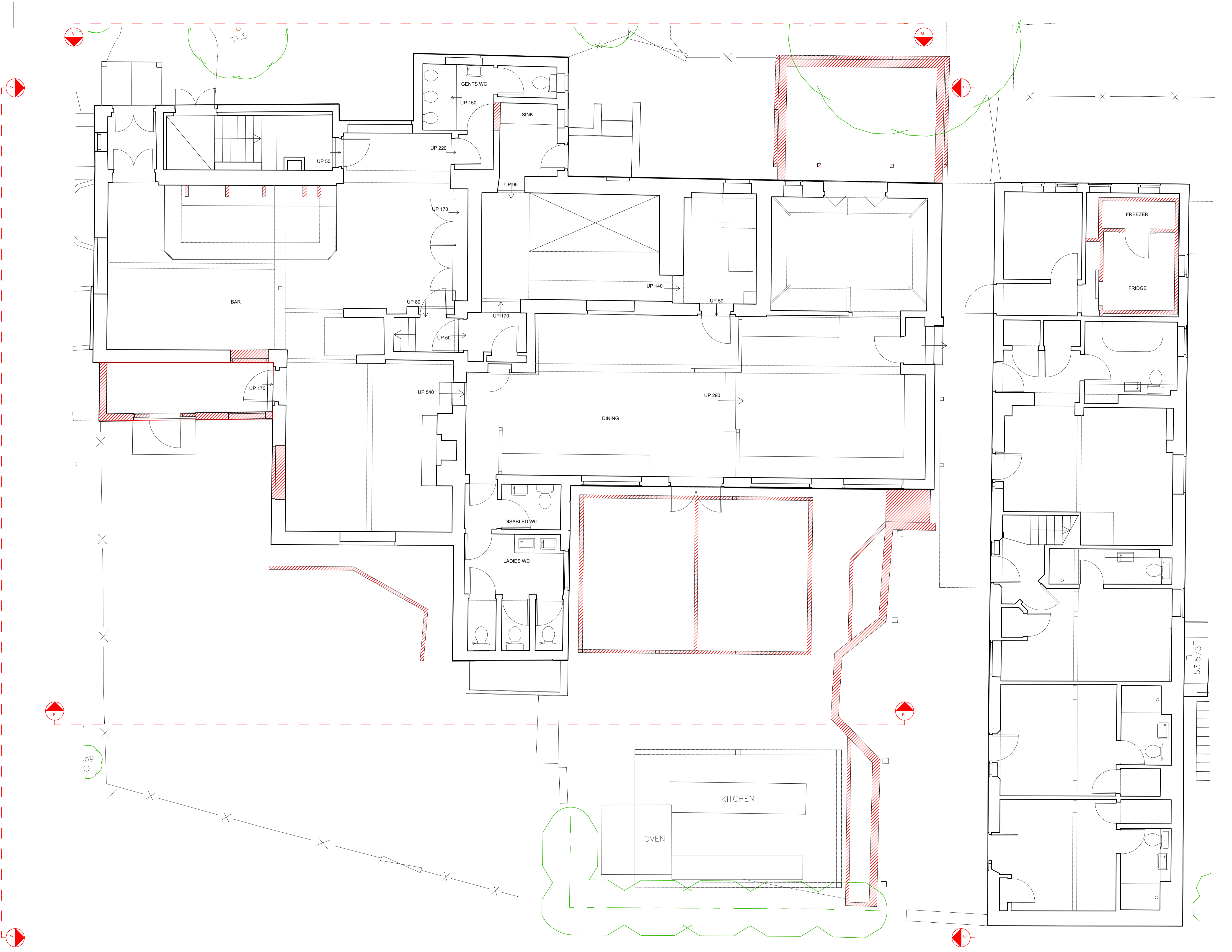
Existing Ground Floor Plan Scale 1:50
