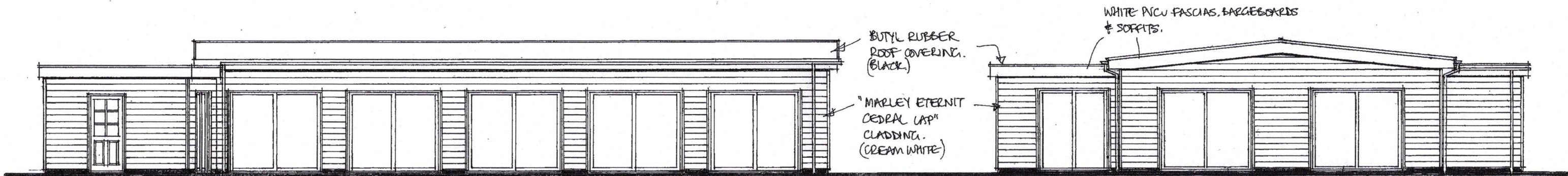
South elevation. 1:100.
