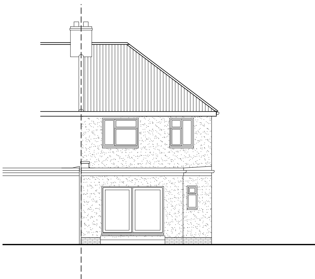
EXISTING REAR (EAST) ELEVATION
