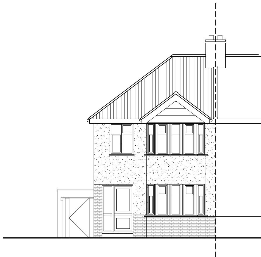
EXISTING FRONT (WEST) ELEVATION
