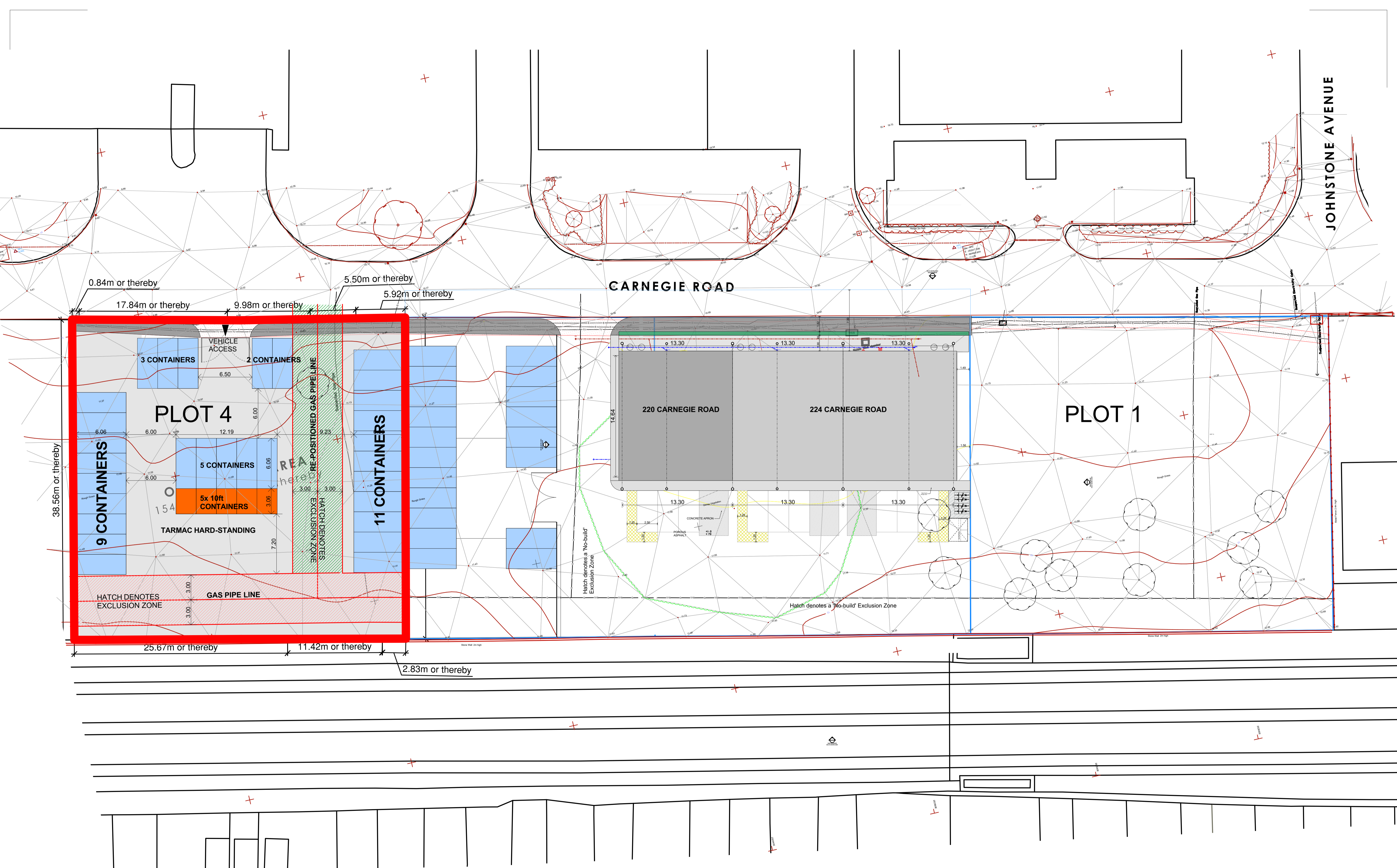
Proposed SPZ Layout 03.10.2023
