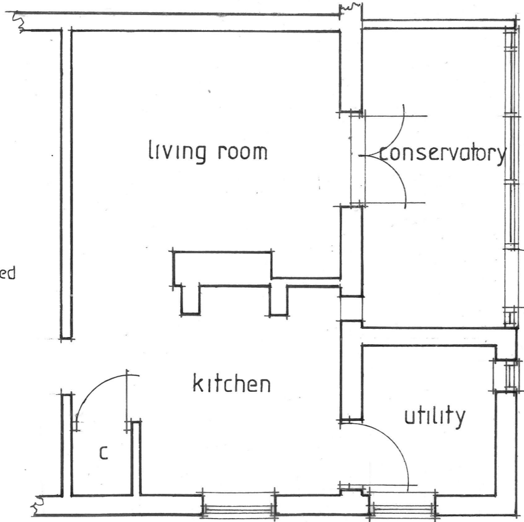
Existing Plan (ATA3) Scales 1:50/1:100
